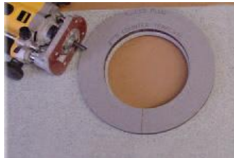
(2) Rout out damage with 12mm(1/2") straight bit 25mm(1") template guide [ 24.3 - A ]
